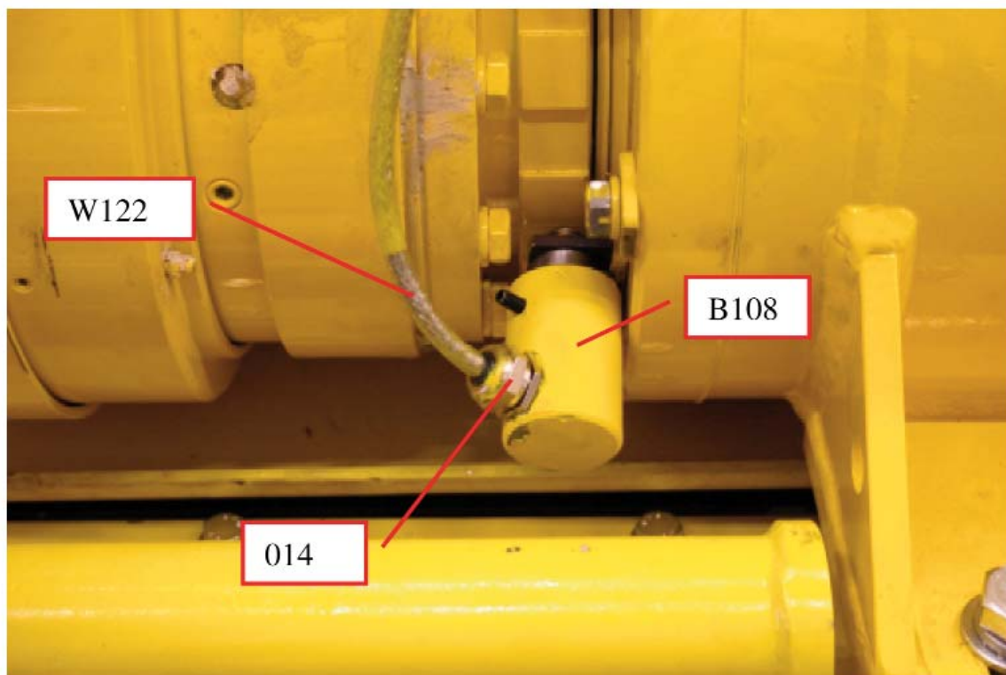
Fig1: Transmitter located on feed unit, see 3719002597
